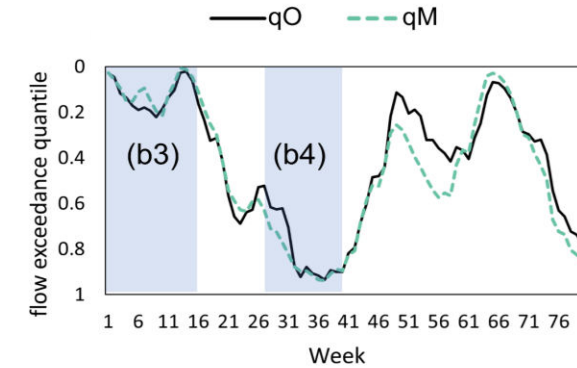
Temporal matching of quantile extremes
