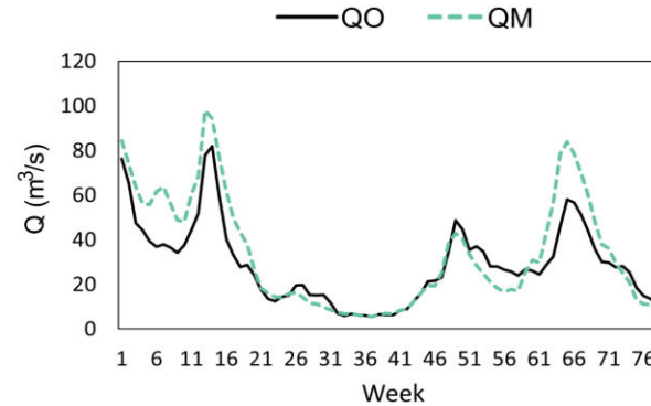
Temporal matching of quantile extremes
